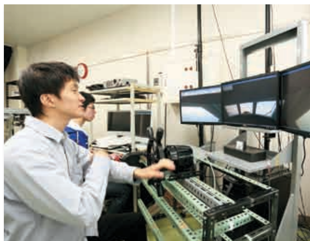
簡易操船シミュレータを用いた小型船舶の操作性評価 Usability Evaluation of Pleasure Boats with Simplified Ship Simulator
